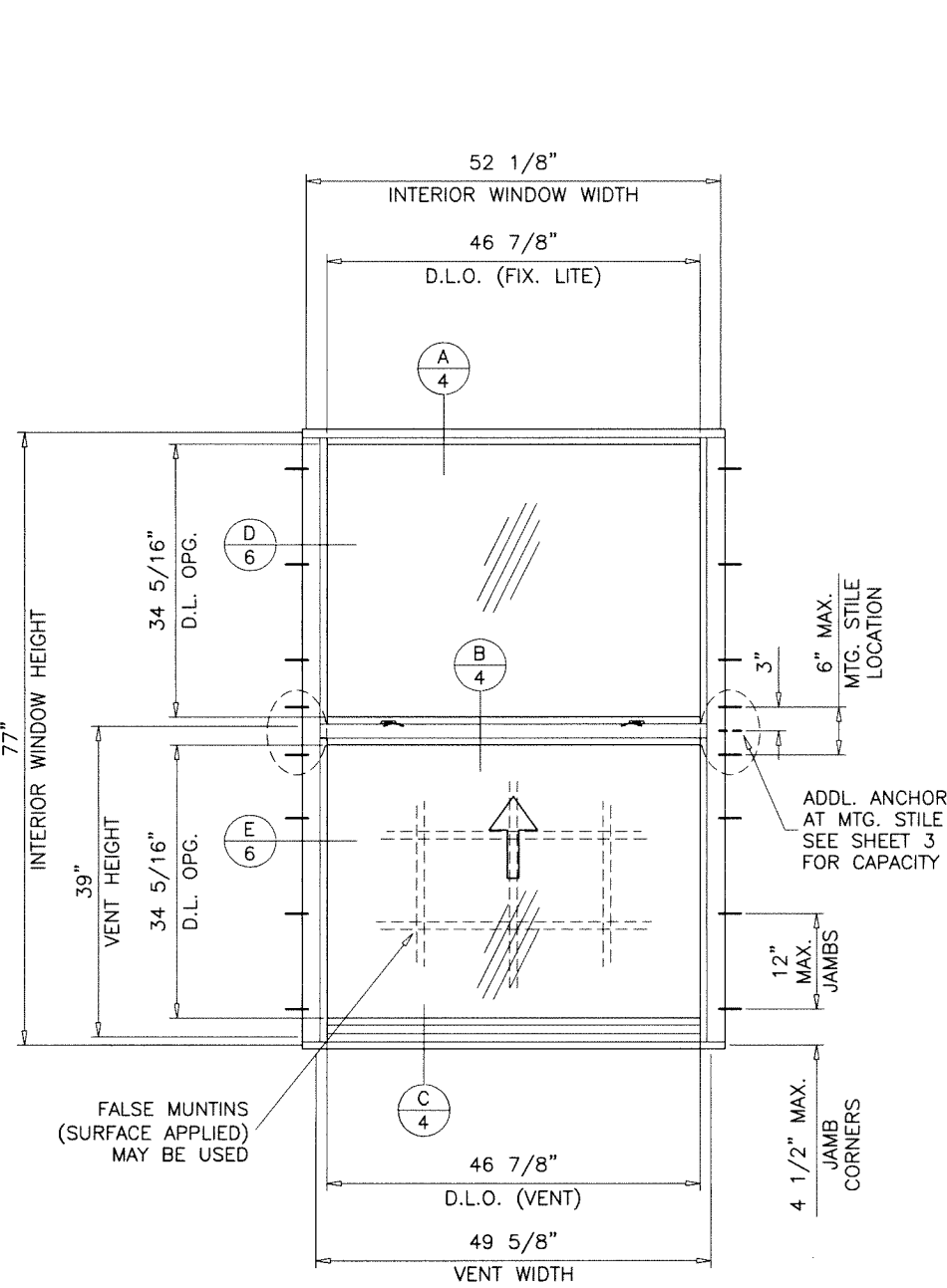
TYPICAL ELEVATION EQUAL LITES
